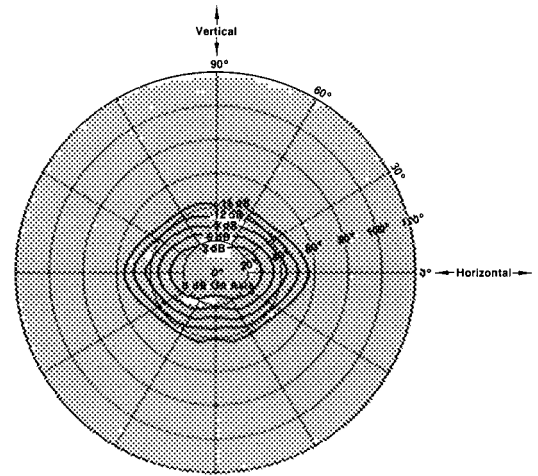
8 kHz octave bandwidth constant sound pressure contours. Same conditions as 500 Hz contours.
