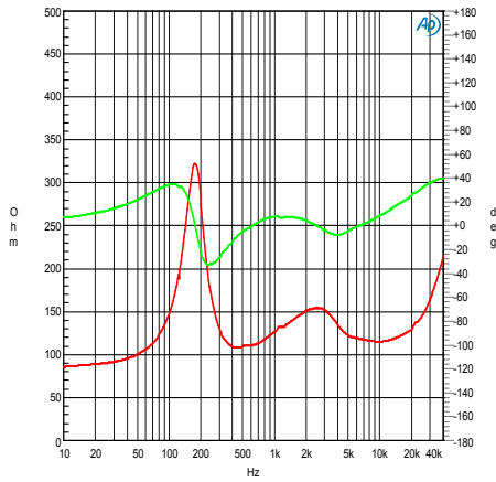
Fig 7 Impedance magnitude (red) and phase (green) vs frequency, 100 W tap / HPF flat / EQ flat.
