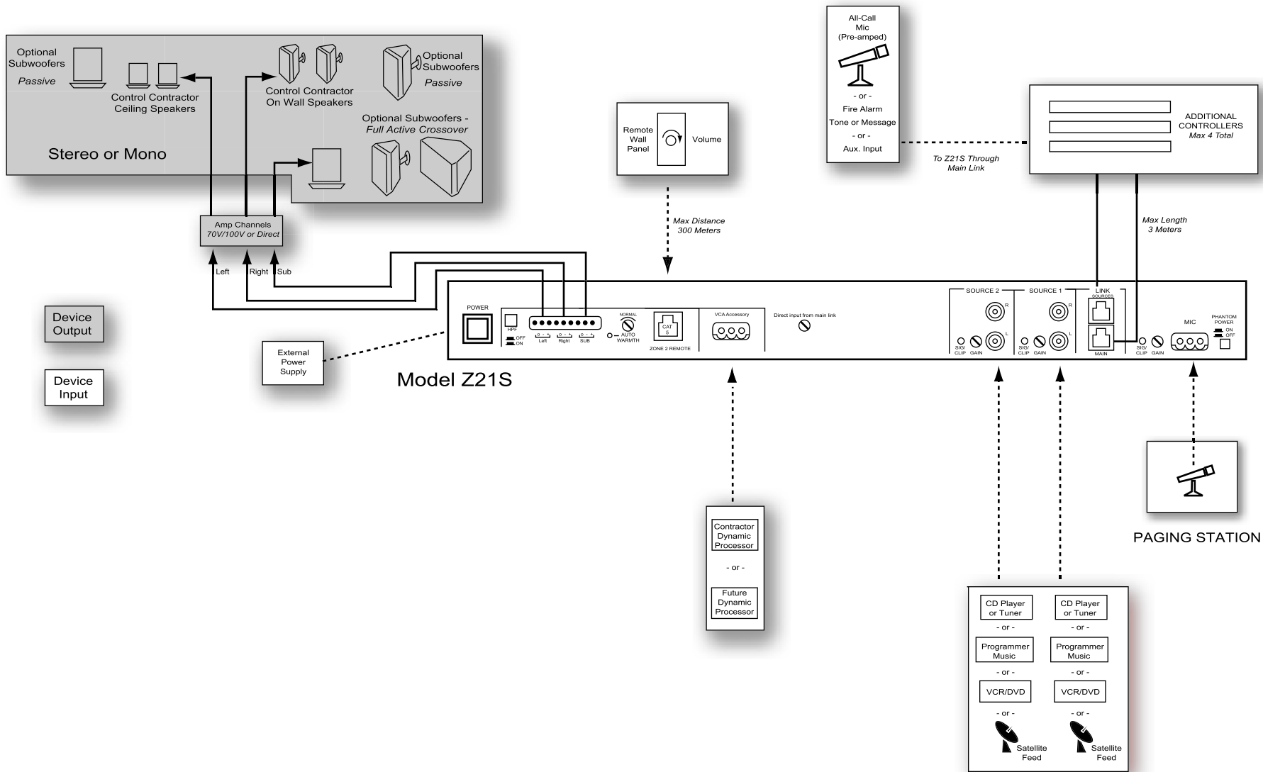
JBL Professional Z21S Controller
