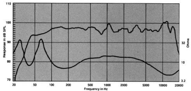
Frequency Response at 1W, 1 meter; Impedance
