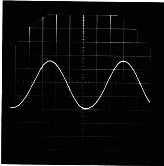
This unretouched photo shows the acoustic output of the system when driven by a 50 W sine wave signal at 35 Hz. A laboratory microphone was used to pick up the sound from the 4311B. The signal from the microphone was connected directly to an oscilloscope and the trace photographed.
