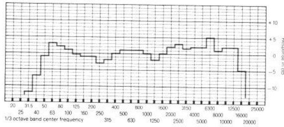
Frequency response of the 4311B taken with \frac{1}{3} -octave band pink noise. Measured at 1 m with a 1-watt input.
