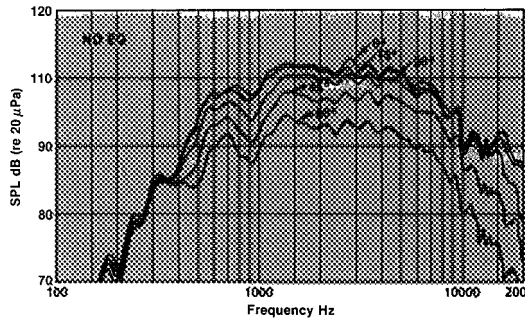
Horizontal off-axis response. Horizontal off-axis response taken at 15 degree intervals out to 60° off axis. Both normalized (equalized flat on axis) and unnormalized responses are shown.
