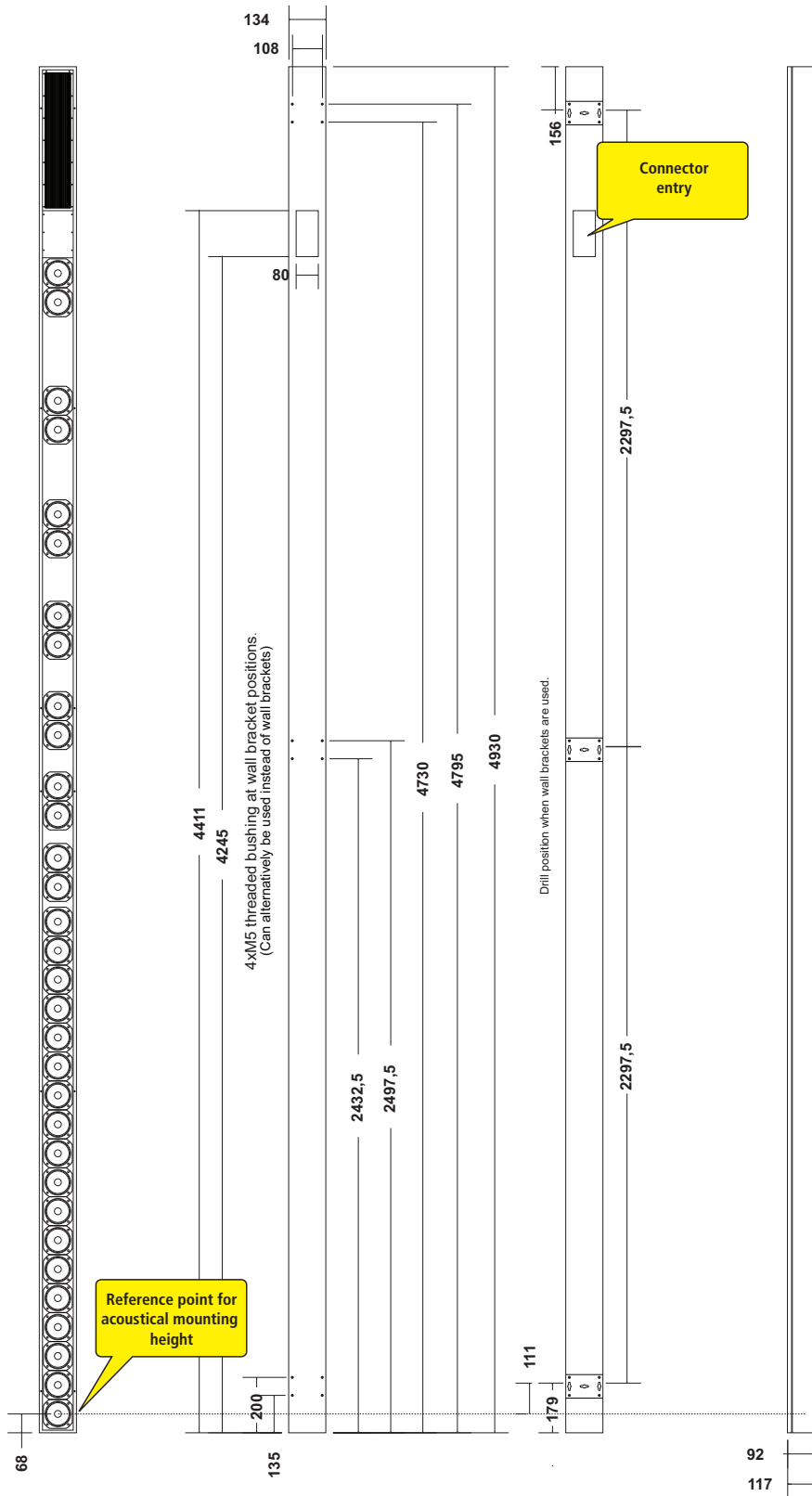
This drawing is valid for the 'amp-at-top' version - part number 585161
